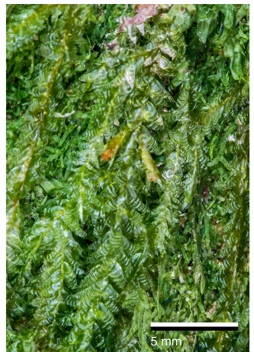
Lower Hutt, Stokes Valley. On Carpodetus serratus . Photographer: Jeremy R. Rolfe, Date taken: 12/12/2017, Licence: CC BY.
